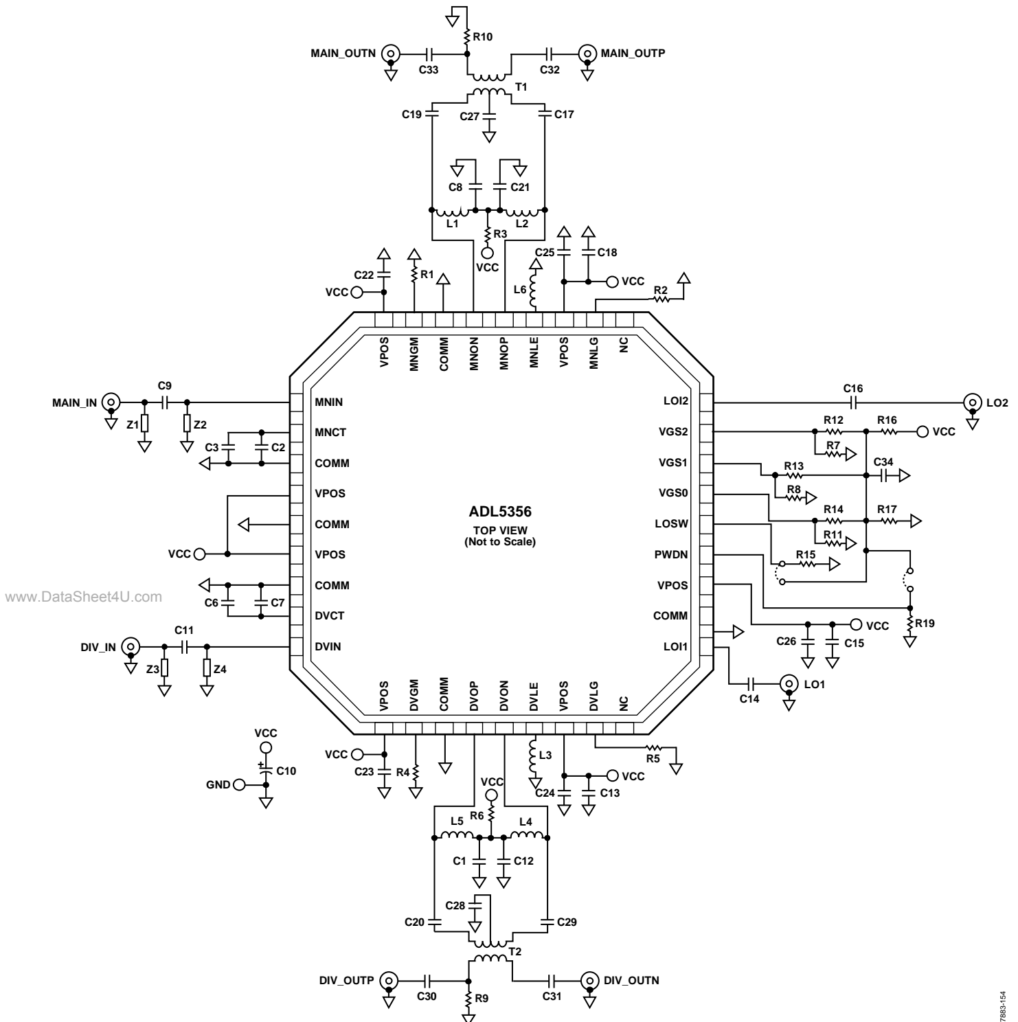
Figure 54. Evaluation Board Schematic
