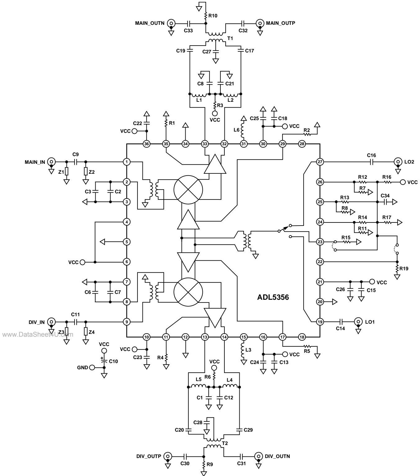
Figure 53. Typical Application Circuit
