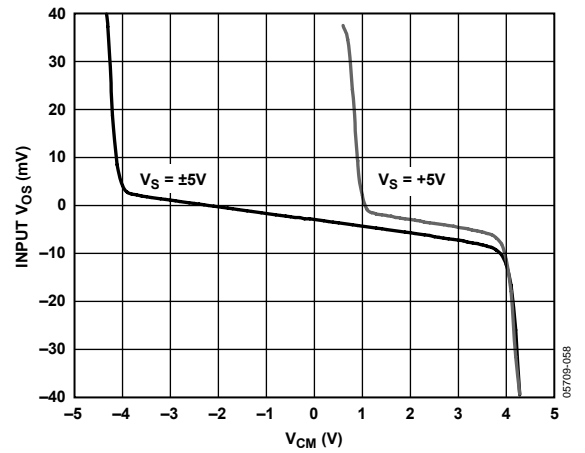
Figure 49. Input V_{Os} vs. Common-Mode Voltage
