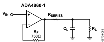
Figure 53. Driving Capacitive Loads
