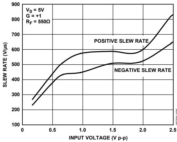
Figure 35. Slew Rate vs. Input Voltage
