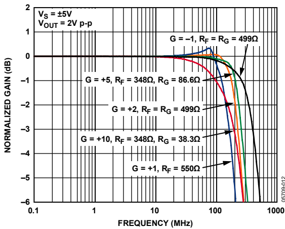
Figure 5. Large Signal Frequency Response for Various Gains
