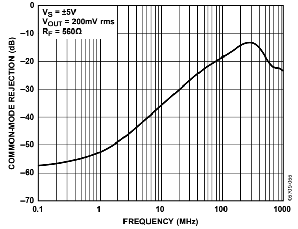
Figure 44. Common-Mode Rejection vs. Frequency
