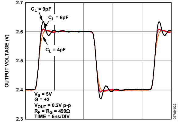
Figure 27. Small Signal Transient Response for Various Capacitor Loads
