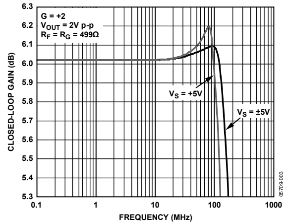
Figure 2. 0.1 dB Flatness
