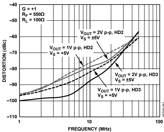
Figure 18. Harmonic Distortion vs. Frequency for Various Supplies
