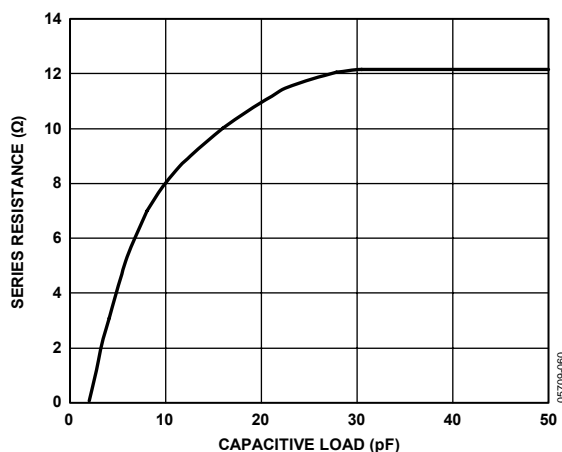
Figure 54. Recommended R_{SERIES} vs. Capacitive Load
