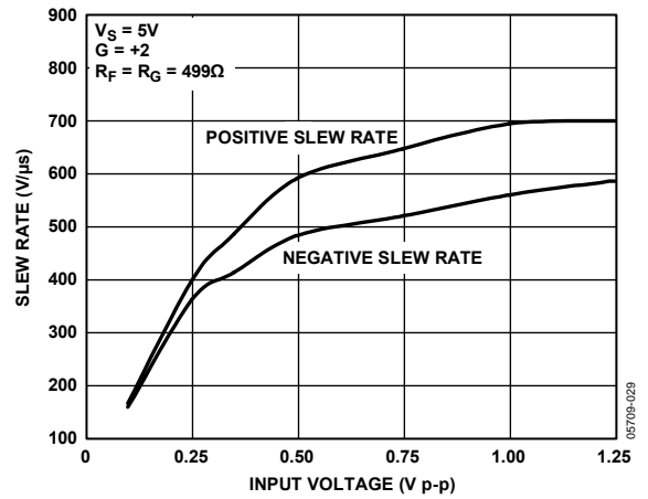
Figure 38. Slew Rate vs. Input Voltage
