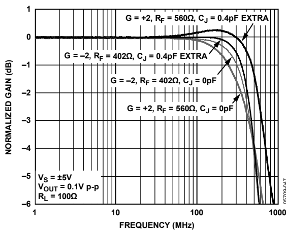
Figure 60. Small Signal Frequency Response vs. Added Summing Junction Capacitance
