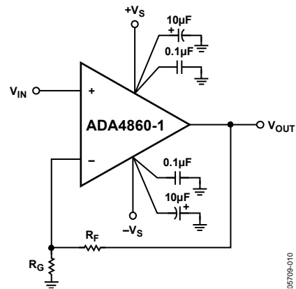
Figure 51. Noninverting Gain
