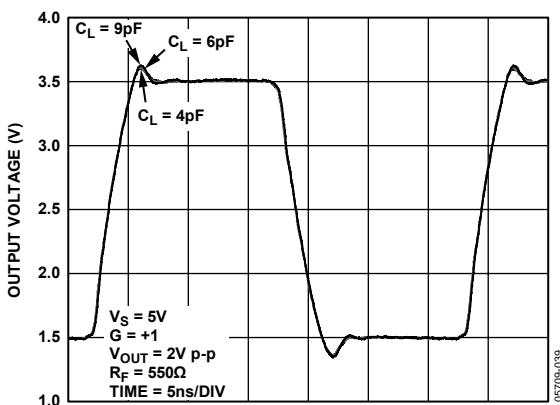
Figure 30. Large Signal Transient Response for Various Capacitor Loads
