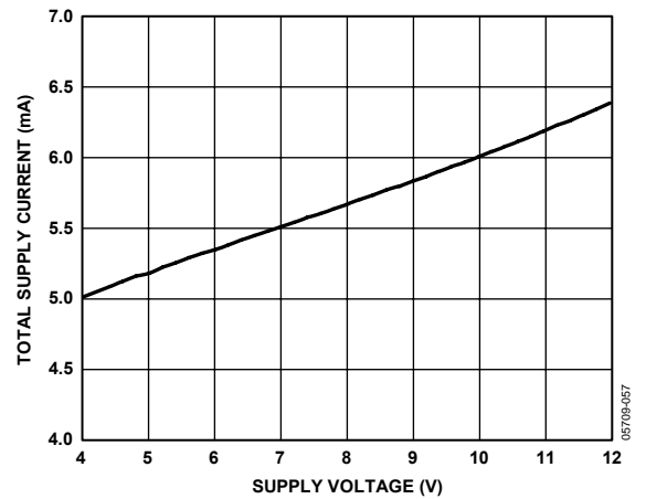
Figure 50. Supply Current vs. Supply Voltage
