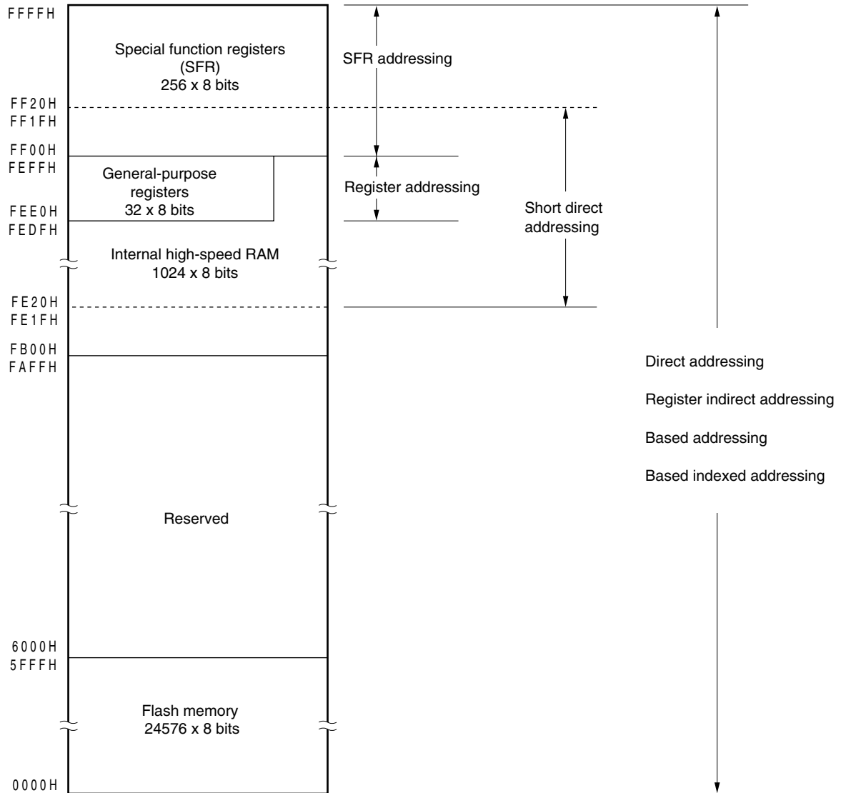
Figure 3-14. Correspondence Between Data Memory and Addressing ( \mu PD78F0502, 78F0502A, 78F0512, 78F0512A, 78F0522, 78F0522A, 78F0532, and 78F0532A)
