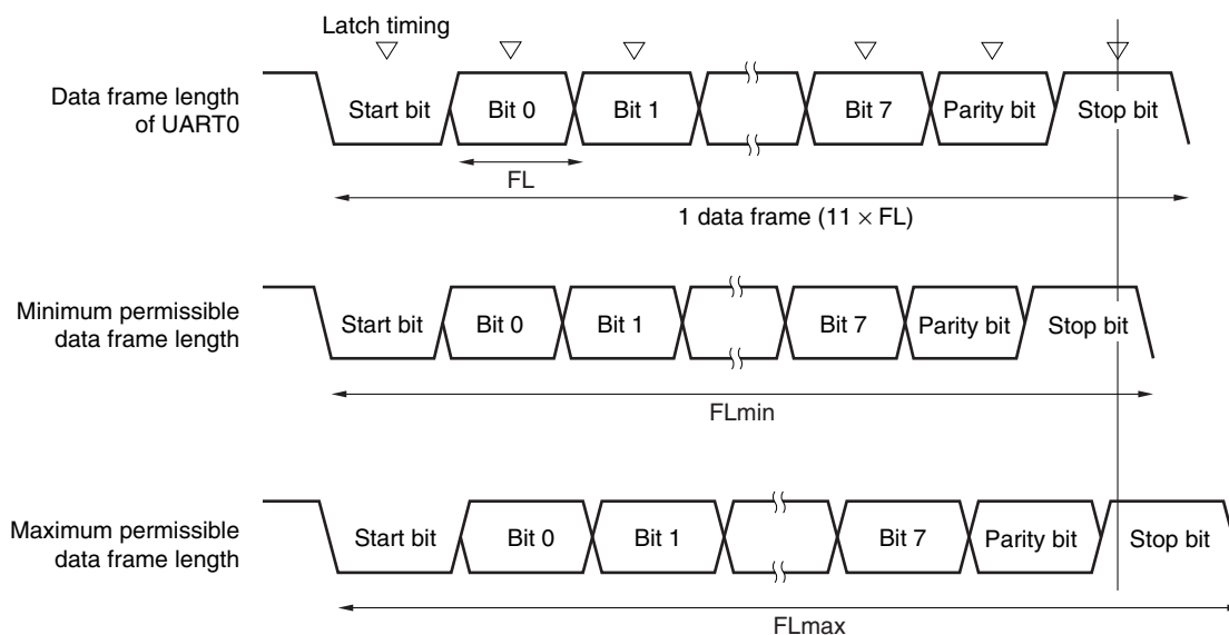
Figure 14-13. Permissible Baud Rate Range During Reception
