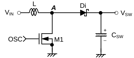
Figure 10 Switching regulator
