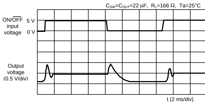
10.4 V_{IN}=3\text{ V} , SEL1=L, SEL2=L
