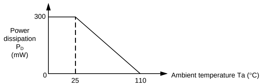
Figure 18 Power dissipation of 8-pin SOP
