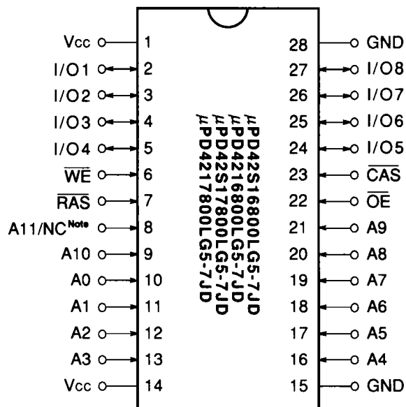
28-pin Plastic TSOP (II)
