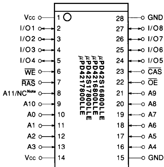
28-pin Plastic SOJ
