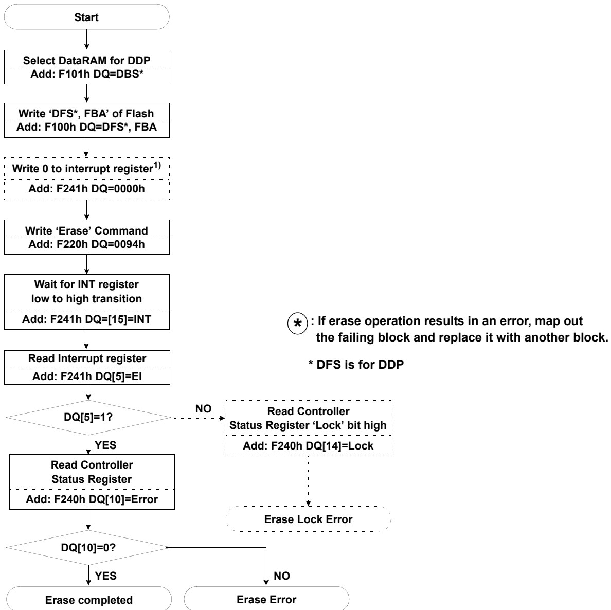
Block Erase Operation Flow Chart
