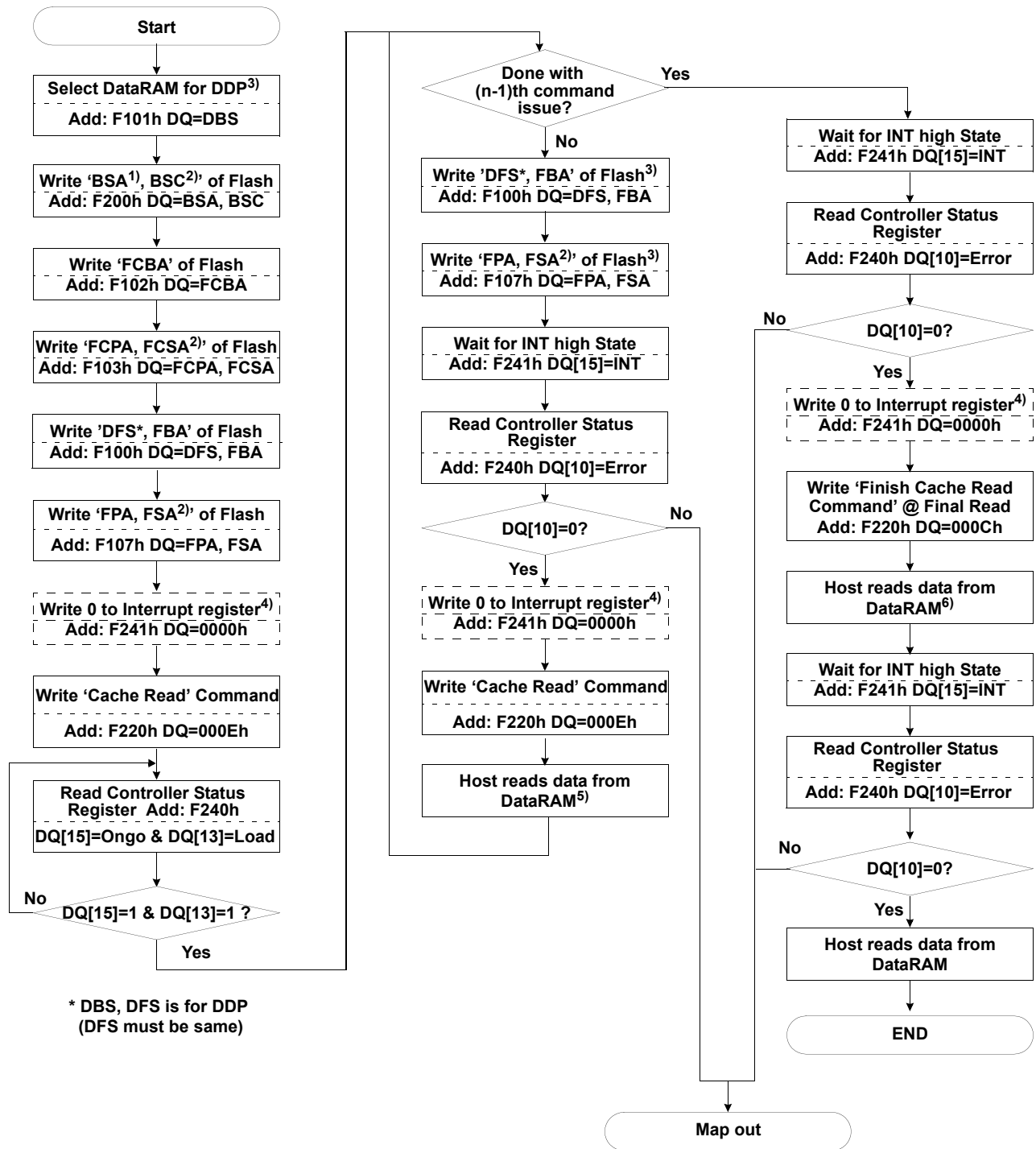
Cache Read Flow Chart
