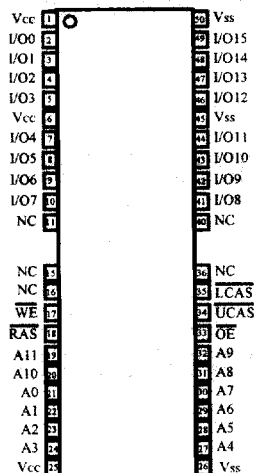
44(50) TSOP II
