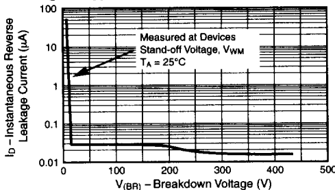
Fig. 7 - Typical Reverse Leakage Characteristics
