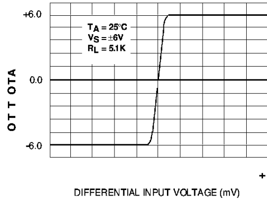
TRANSFER FUNCTION
