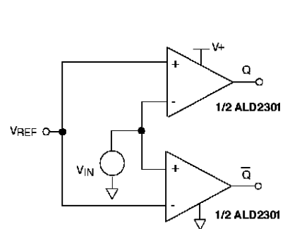
VOLTAGE COMPARATOR WITH COMPLEMENTARY OUTPUTS
