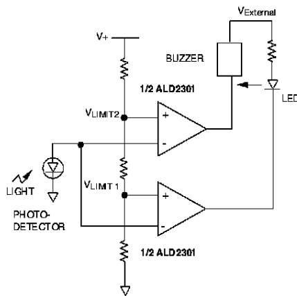
DUAL LIMIT PHOTO-DETECTOR MONITOR
