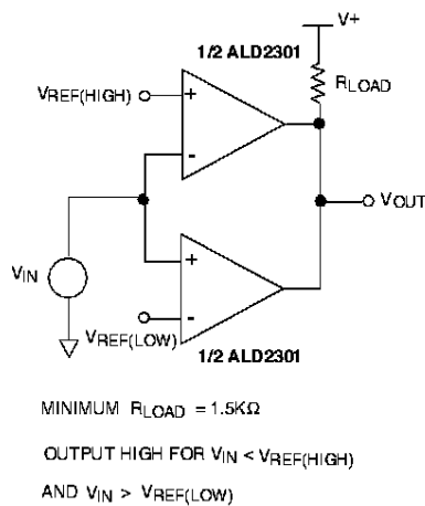
DUAL LIMIT WINDOW COMPARATOR
