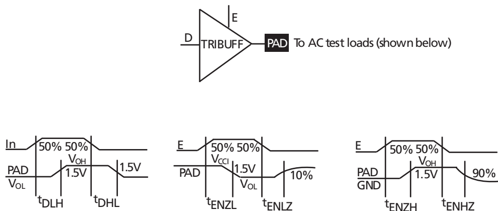
Figure 1-21 • Output Buffer Delays
