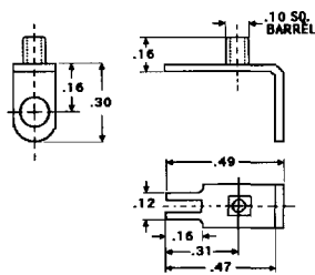
BRACKETS (MINIATURE)
