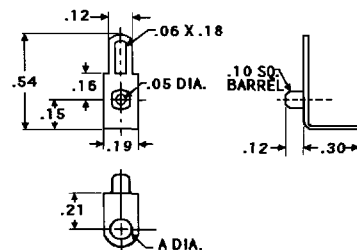
MOUNTING LUGS (MINIATURE)
