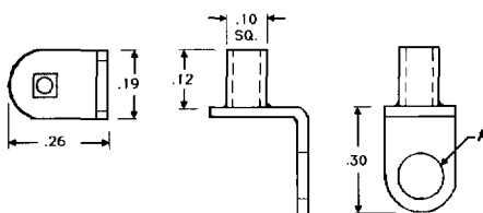
DRAWN LUGS (MINIATURE)
