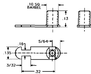
DRAWN LUGS (MINIATURE)
