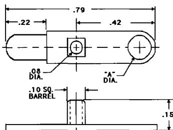
STRAIGHT (MINIATURE)
