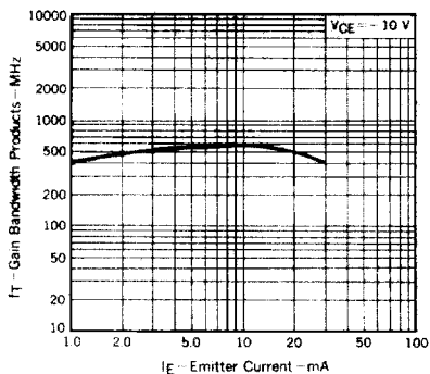
GAIN BANDWIDTH PRODUCTS vs. EMITTER CURRENT
