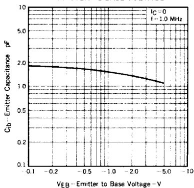
INPUT CAPACITANCE vs. EMITTER TO BASE VOLTAGE
