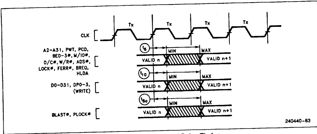
Figure 13.5. Output Valid Delay Timing
