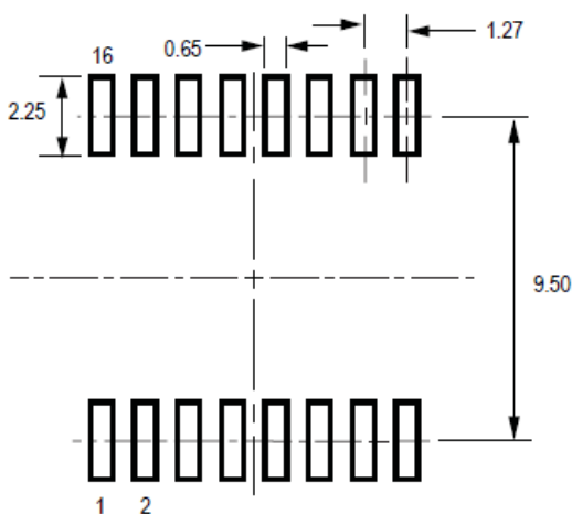
C PCB Layout Reference View
