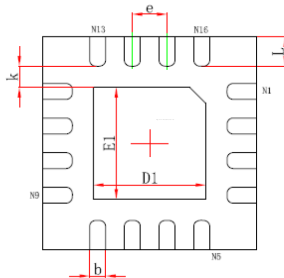
<QFN -16> Bottom View
