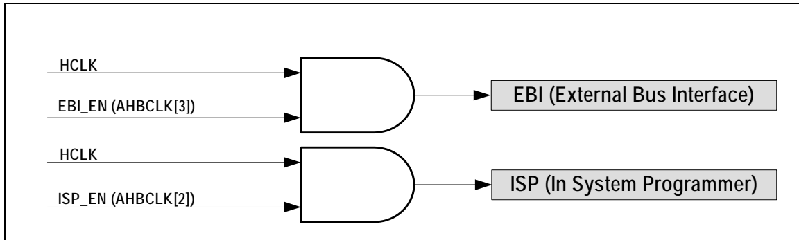
Figure 6–6 AHB Clock Source for HCLK
