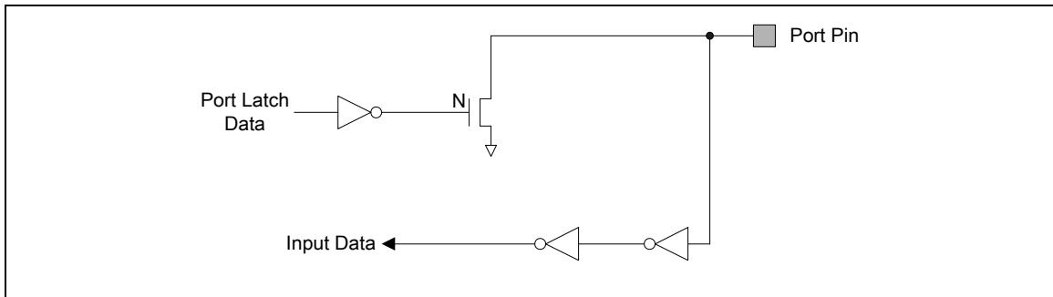
Figure 6-11 Open-Drain Output
