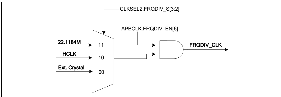
Figure 6–8 Clock Source of Frequency Divider
