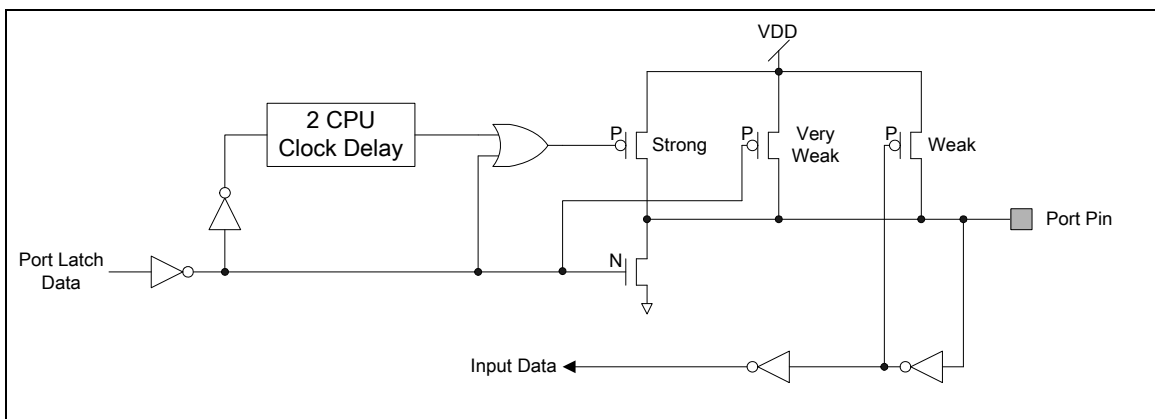
Figure 6-12 Quasi-bidirectional I/O Mode
