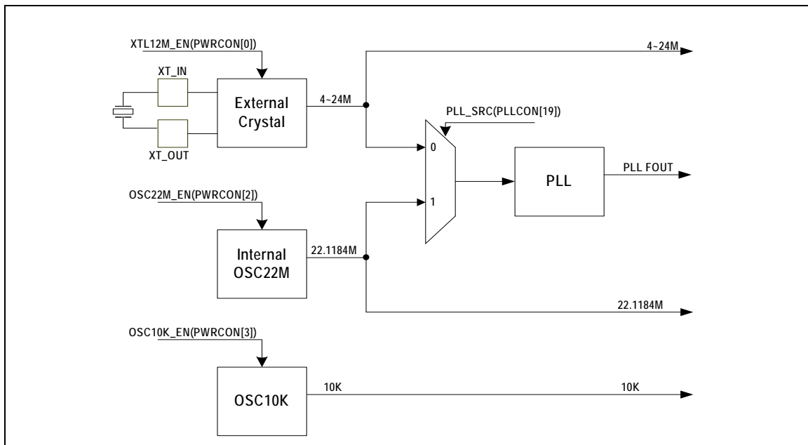
Figure 6–3 Clock generator block diagram
