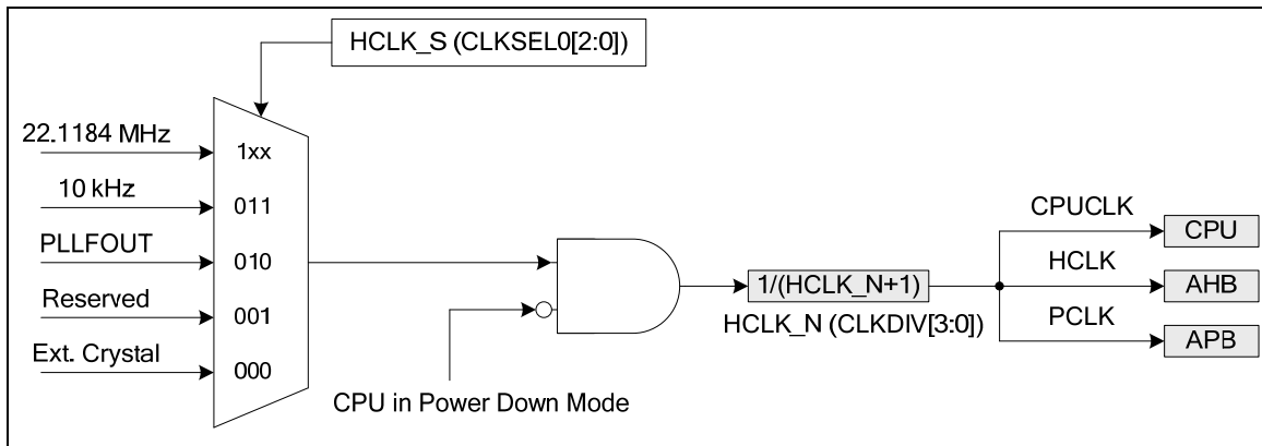
Figure 6–4 System Clock Block Diagram
