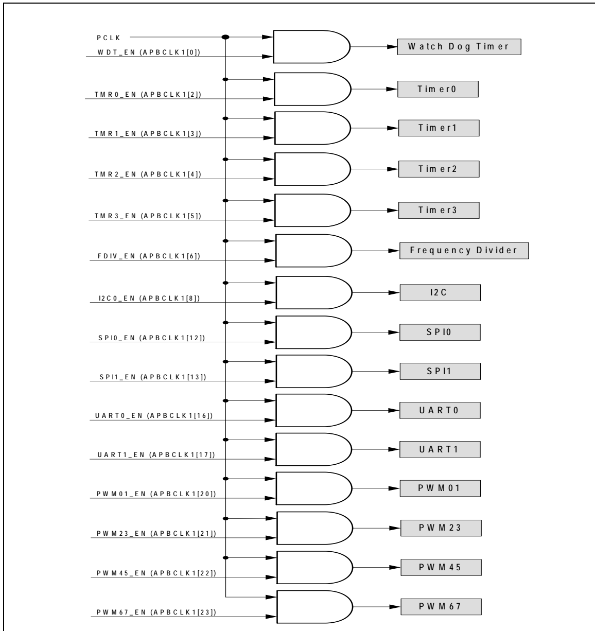
Figure 6-7 Peripherals Clock Source Select for PCLK
