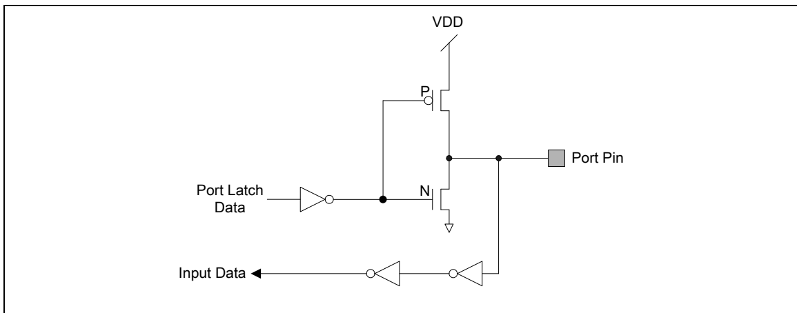
Figure 6–10 Push-Pull Output
