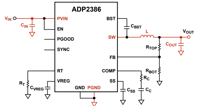
Figure 35. High Current Path in the PCB Circuit
