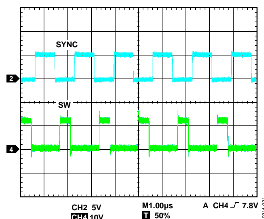
Figure 21. External Synchronization
