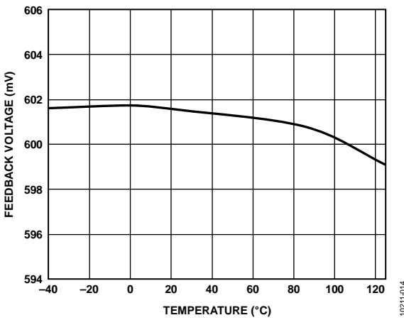
Figure 14. Feedback Voltage vs. Temperature
