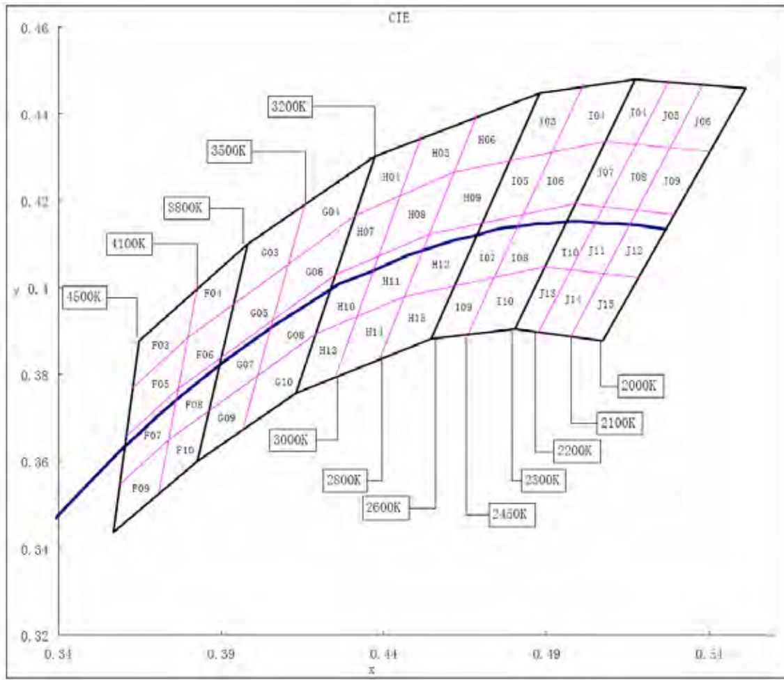
*Bin Range of Chromaticity Coordinates (OSW35630C1A)
