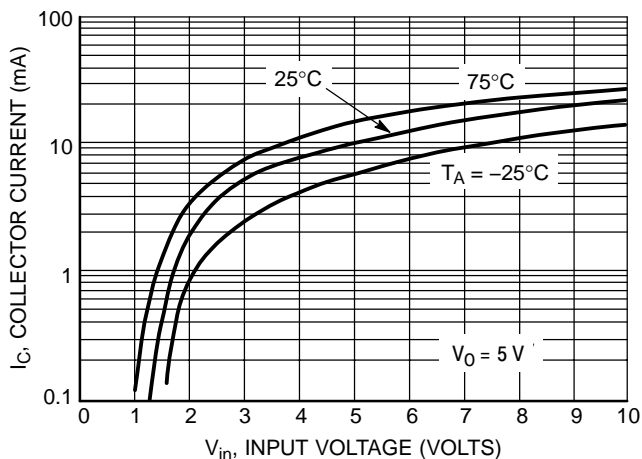
Figure 65. Output Current versus Input Voltage
