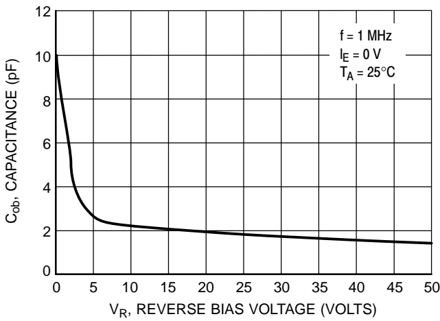
Figure 29. Output Capacitance
