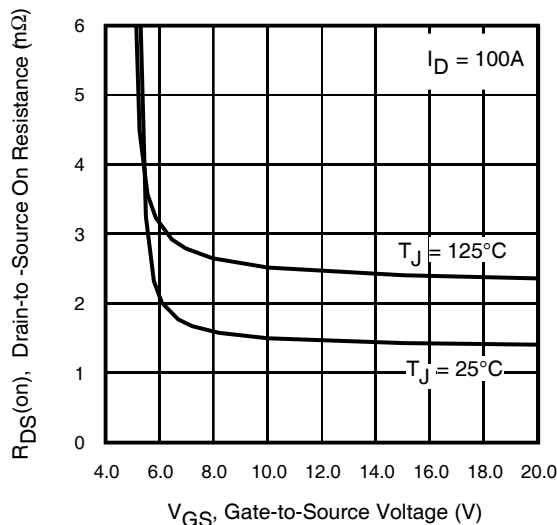
Fig 1. Typical On-Resistance vs. Gate Voltage www.irf.com
