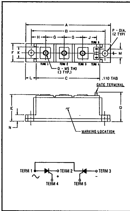
1200-1600 Volts CD4A ___ 90 Outline Drawing
