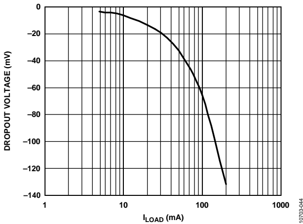
Figure 44. Dropout Voltage vs. Load Current ( I_{LOAD} ), Adjustable Output Voltage, V_{OUT} = -15 V
