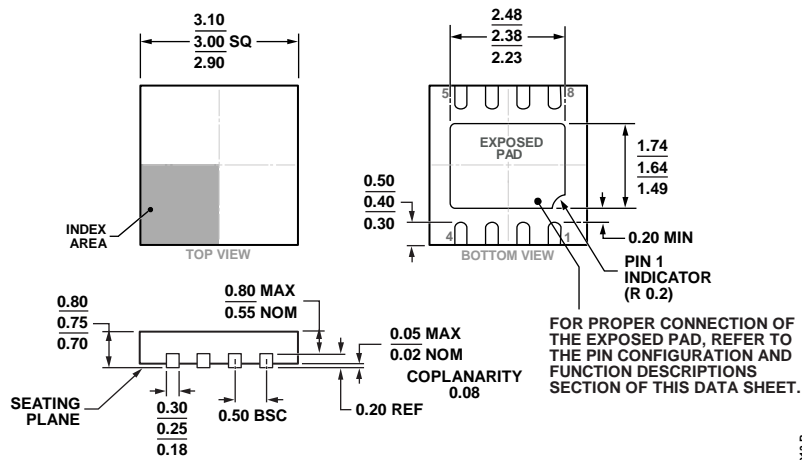
Figure 97. 8-Lead Lead Frame Chip Scale Package [LFCSP_WD] 3 mm × 3 mm Body, Very Very Thin, Dual Lead (CP-8-5) Dimensions shown in millimeters
