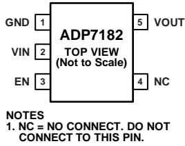
Figure 3. 5-Lead TSOT Pin Configuration, Fixed Output Voltage
