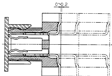
SECT. X-X
