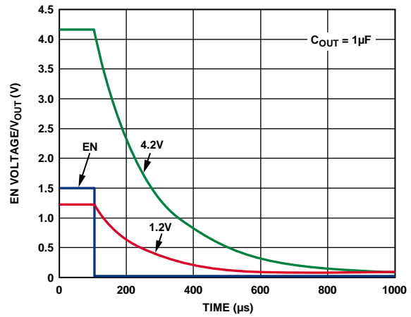
Figure 40. Typical Shutdown Behavior, No Load (ADP160/ADP161)
