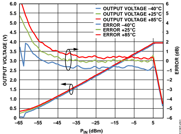
Figure 53. 2.14 GHz V_{RMS} and Log Conformance Error at +25^\circ\text{C} , -40^\circ\text{C} , and +85^\circ\text{C} Using Two-Point Calibration at 0 dBm and -40 dBm
