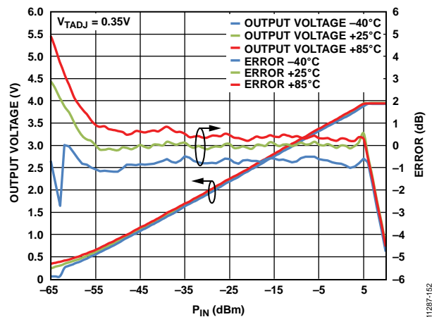
Figure 54. 2.14 GHz V_{RMS} and Log Conformance Error at +25^\circ\text{C} , -40^\circ\text{C} , and +85^\circ\text{C} Using Three-Point Calibration at 0 dBm, -40 dBm, and -55 dBm
