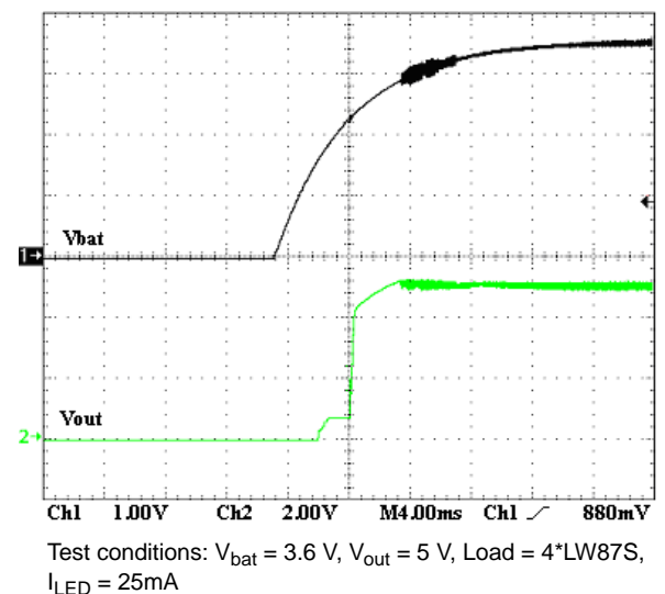
Figure 8. Output Voltage Startup from Scratch
