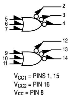
Figure 1. Logic Diagram
