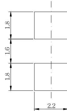
Recommended Solder Pattern
