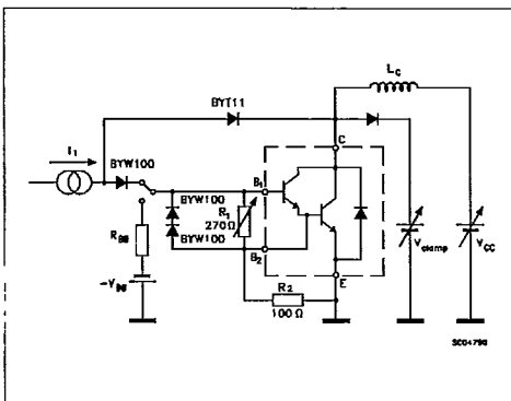
Turn-off Switching Test Circuit
