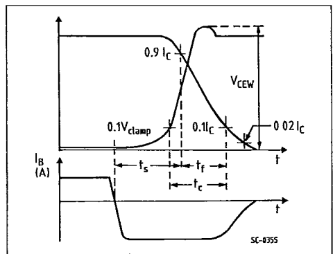
Turn-off Switching Waveforms
