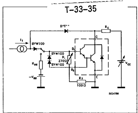
Turn-on Switching Test Circuit
