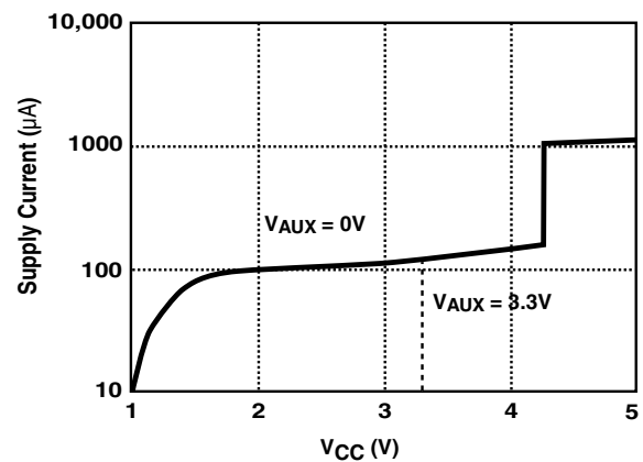
Figure 4. V_{CC} Supply Current (No Load).
