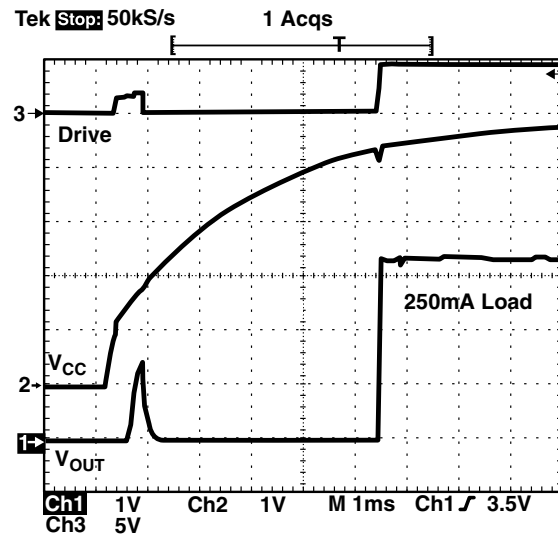
Figure 5. V_{CC} Power-up Cold Start
