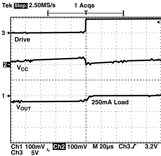
Figure 6. V CC Power-up (V AUX = 3.3V)
