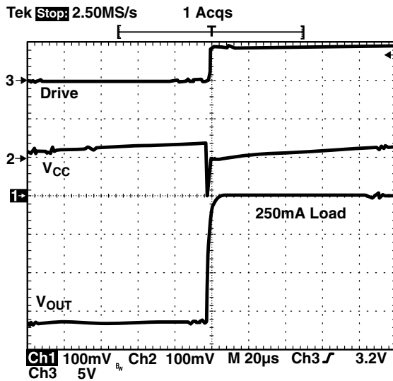
Figure 7. V CC Power-up (V AUX = 3.0V).
