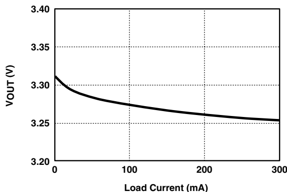
Figure 2. Load Regulation
