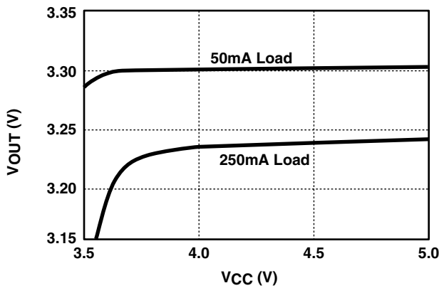
Figure 1. Dropout Characteristics
