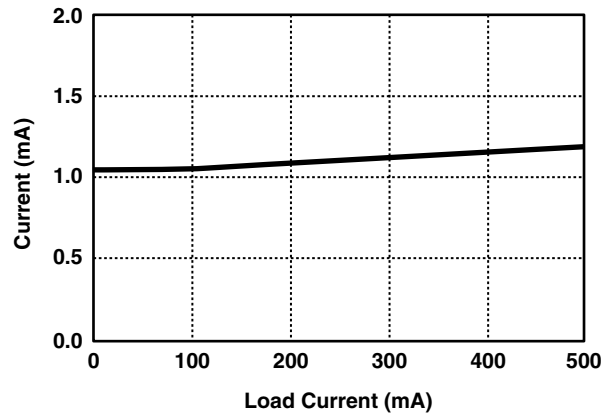
Figure 3. Ground Current
