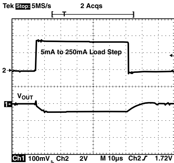
Figure 10. Load Step Response.
