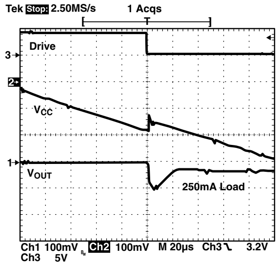
Figure 8. V CC Power-down (V AUX = 3.3V).
