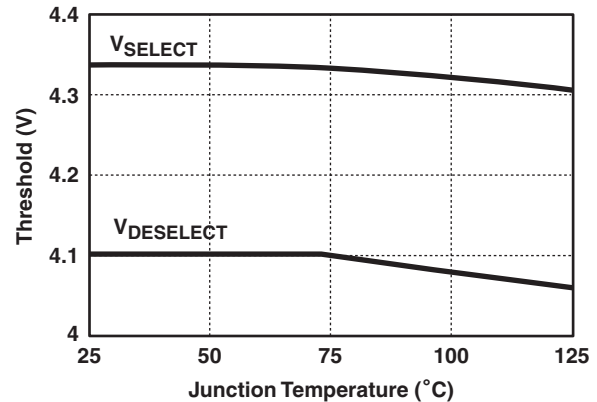
Figure 13. Threshold vs. Temperature.
