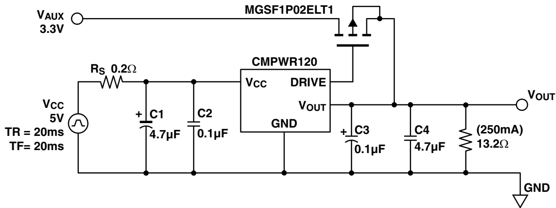
Transient Characteristics Test Setup
