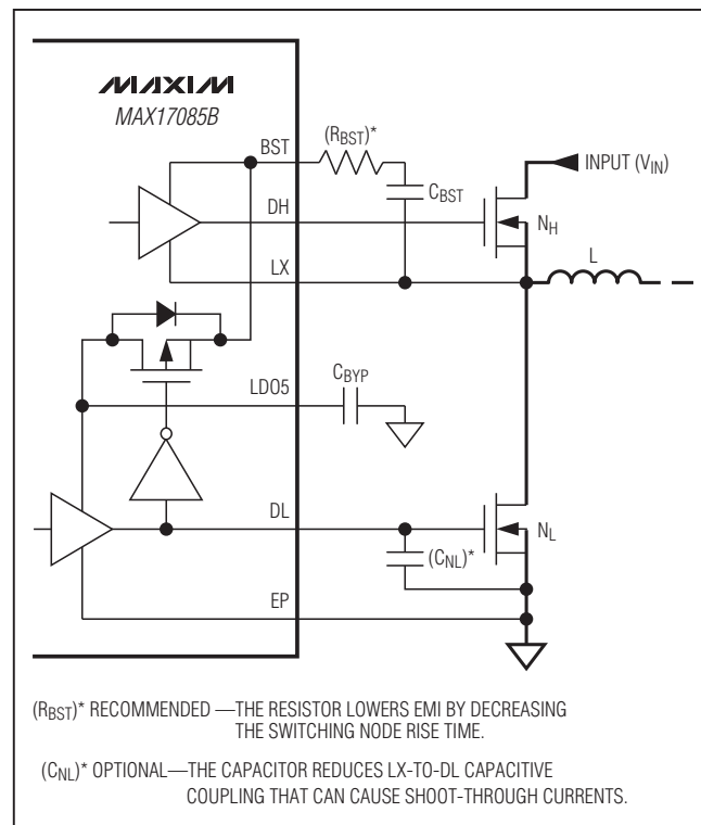
Figure 7. Gate-Drive Circuit
