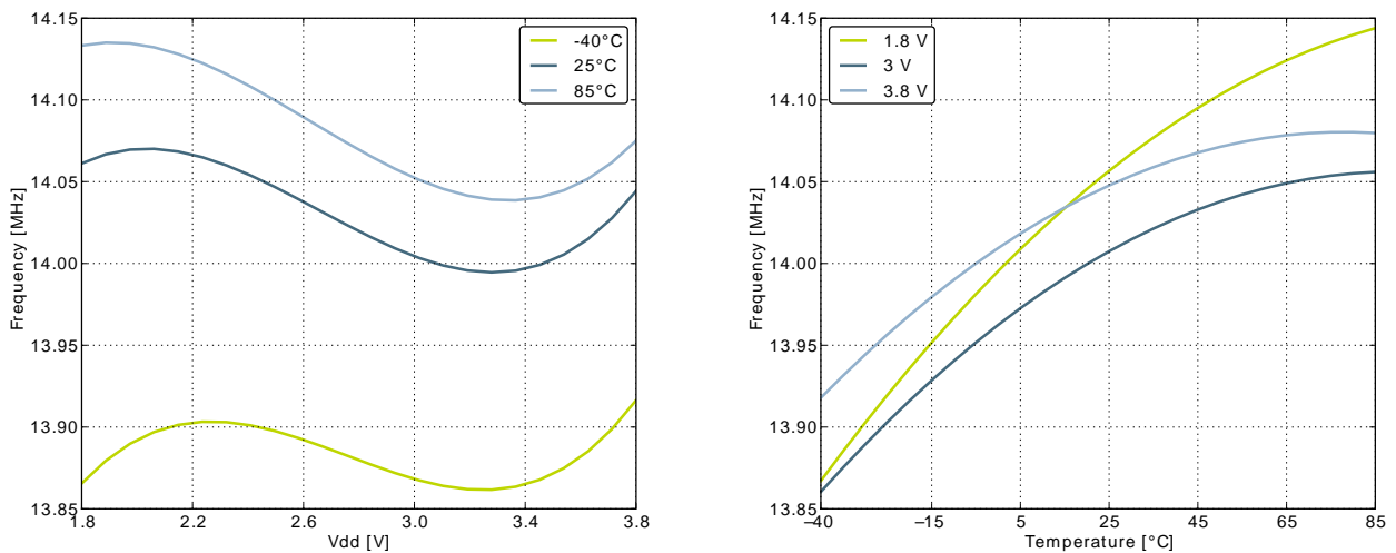
Figure 3.26. Calibrated HFRCO 21 MHz Band Frequency vs Temperature and Supply Voltage
