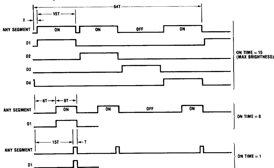
FIGURE 5. Segment and Digit Output Timing Diagram
