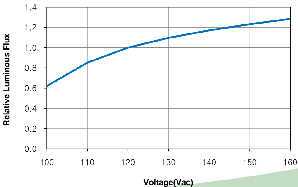
Relative Luminous Flux vs. Voltage at Ta=25 °C
