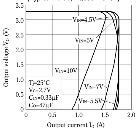
Fig.7 Overcurrent Protection Characteristics (Typical Value, PQ033EF01SZ)
