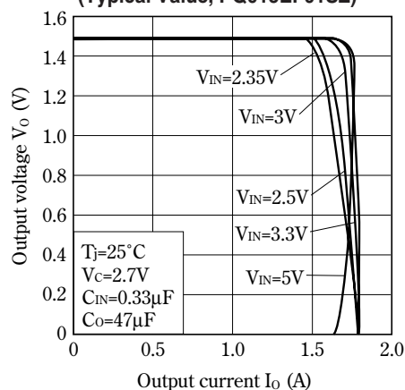
Fig.6 Overcurrent Protection Characteristics (Typical Value, PQ025EF01SZ)
