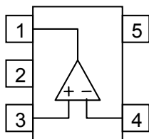
SOT-23-5, SC88A (Top View)
