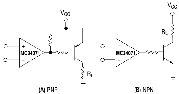
Figure 47. Transistor Driver
