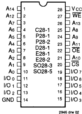
DIP/SOJ/SOIC TOP VIEW
