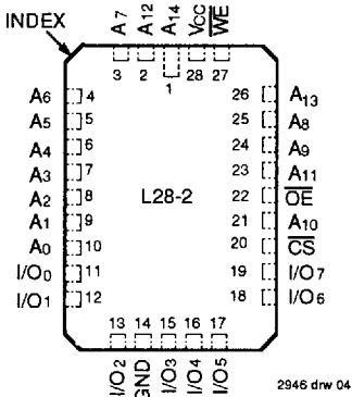
28-Pin LCC TOP VIEW
