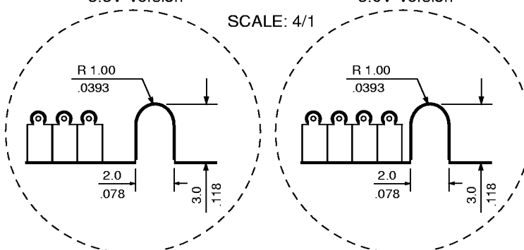
Detail A 3.3V Version
