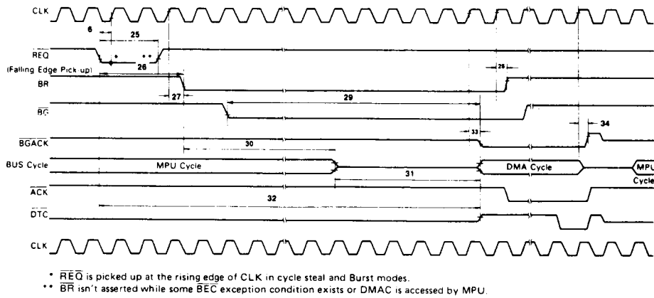
Figure 4 AC Electrical Waveforms – Bus Arbitration
