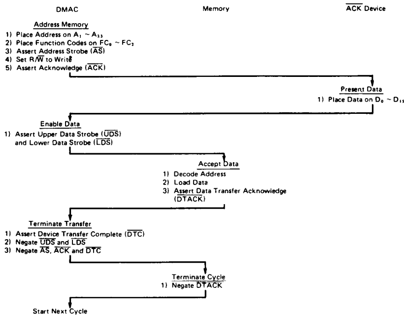
Figure 29 Word from Device with \overline{\text{ACK}} to Memory
