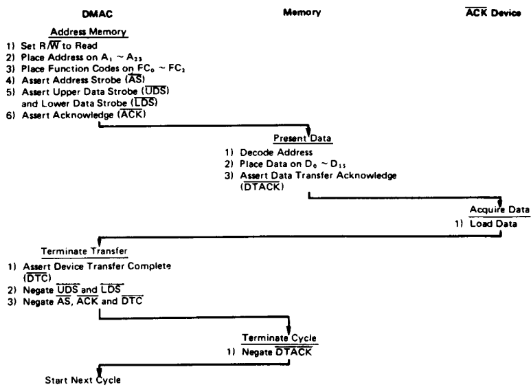
Figure 28 Word from Memory to Device with \overline{\text{ACK}}
