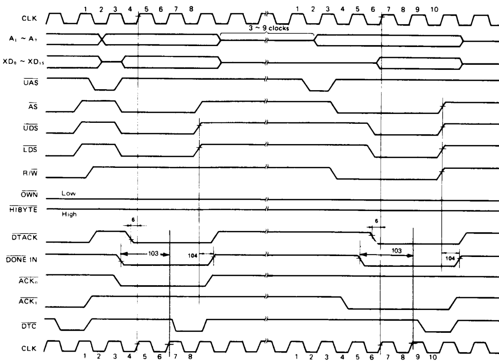
Figure 8 AC Electrical Waveforms – \overline{DONE} Input
