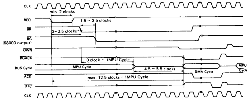
Figure 13 DMAC Bus Arbitration Timing
