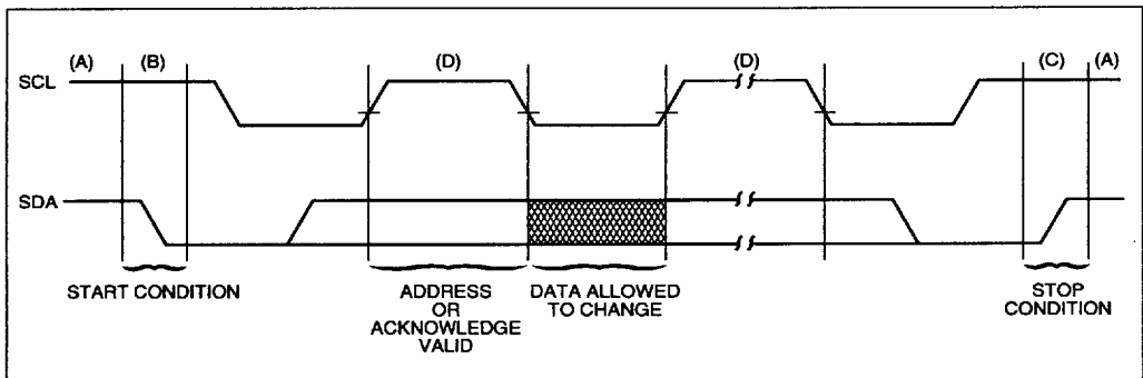
FIGURE 1 - DATA TRANSFER SEQUENCE ON THE SERIAL BUS
