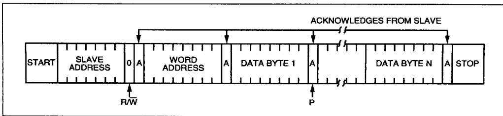
FIGURE 3 - PROGRAM MODE (ERASE/WRITE)
