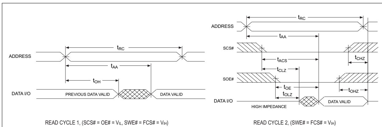
FIGURE 3 – SRAM TIMING WAVEFORM - READ CYCLE
