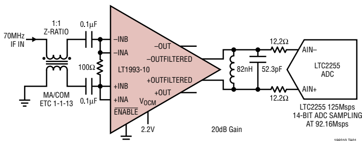
4-Channel WCDMA Receive Channel
