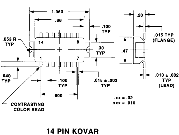
14 PIN KOVAR
