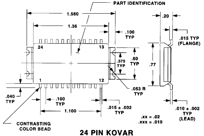
24 PIN KOVAR
