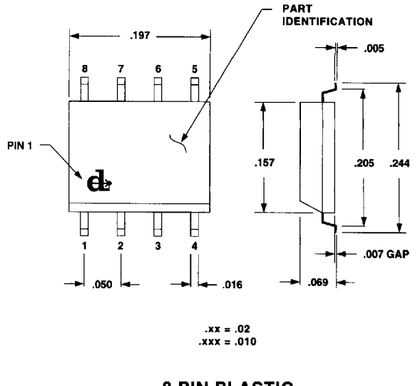
8 PIN PLASTIC
