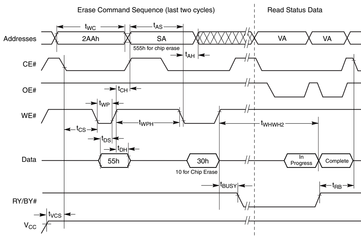
Figure 18. Chip/Sector Erase Operation Timings
