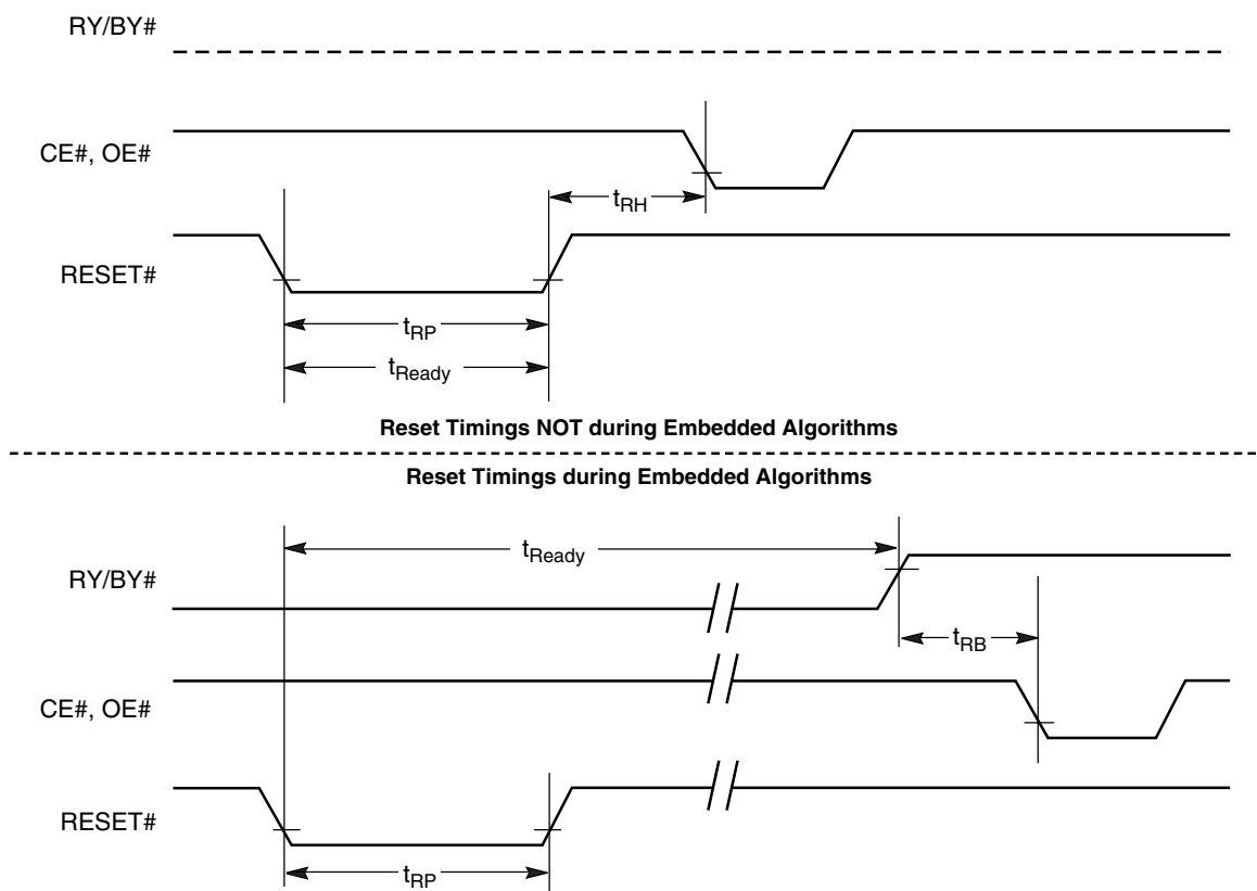
Figure 15. Reset Timings
