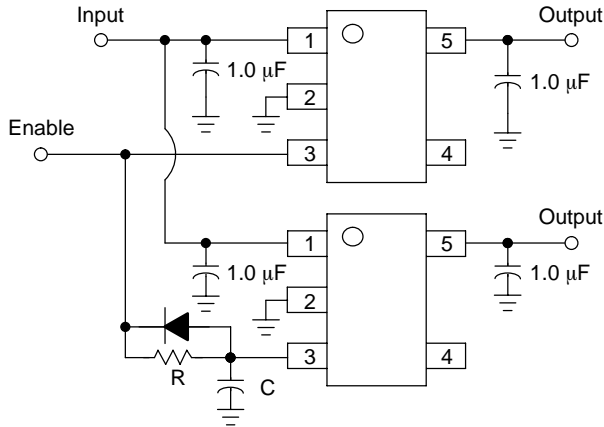
Figure 32. Delayed Turn-on
