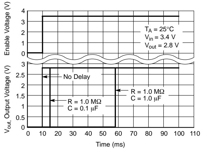
Figure 33. Delayed Turn-on
