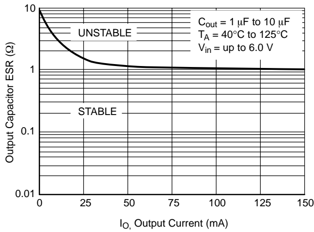
Figure 29. Stability
