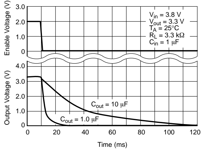
Figure 23. Turn-off Response
