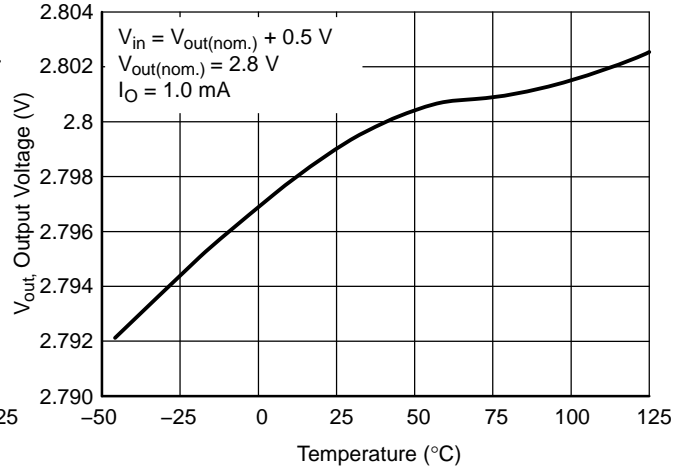
Figure 9. Output Voltage vs. Temperature
