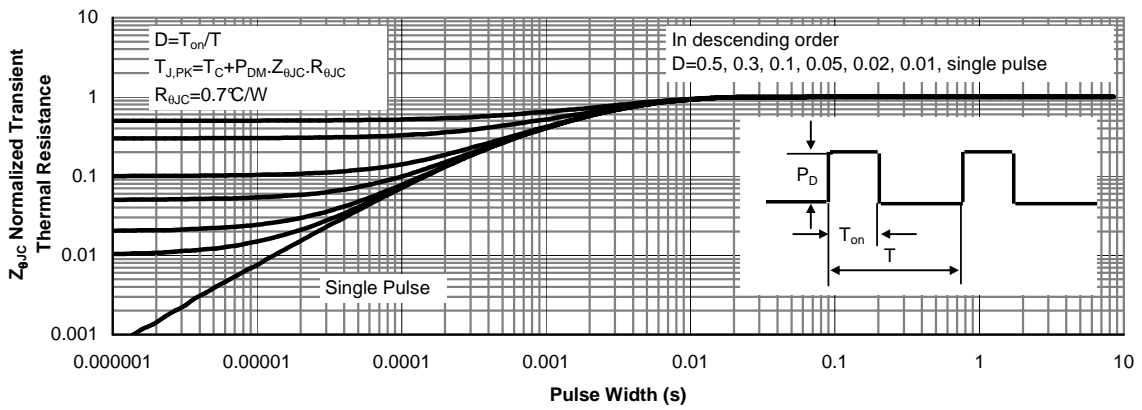
Figure 15: Normalized Maximum Transient Thermal Impedance for AOW11S60 (Note F)
