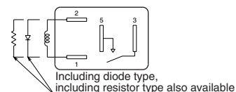
Schematic (Bottom view) 1 Form A
