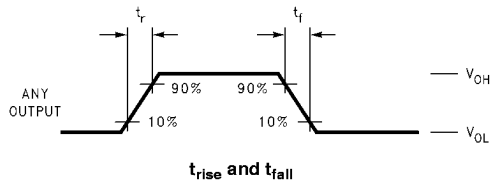
FIGURE 2. Waveforms (Input Pulse Characteristics; f=1MHz, t_r=t_f=3ns )
